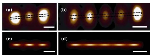
Figure 8. TPI-PL images for single gold nanorods: (a) 20 \pm 5 nm \times 330 \pm 30 nm, (b) 20 \pm 5 nm \times 540 \pm 40 nm. (c,d) Calculated LDOS maps for corresponding gold nanorods (a,b), respectively. Scale bars are 100 nm. (Reproduced with permission from ref. 20. Copyright 2005, American Chemical Society.)
